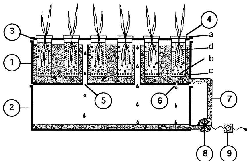
Figure 1. Diagram of the automatic immersion system (immersion phase) used for the multiplication of single cystosorus strains of Polymyxa sp. 1) Upper culture tank; 2) lower reservoir tank; 3) removable opaque lid on the upper tank with openings for insertion of culture tubes; 4) culture tube with (a) 32 mm ring (internal diameter) sealed to the tube, (b) a polyamid netting sealed to the tube with a 32 mm ring (external diameter) (c) and supporting the sand inoculum mixture (d); 5) overflow tubes sealed to the bottom of the culture tank; 6) emptying hole; 7) PVC tubing; 8) centrifugal pump; 9) timer for regulation of the alternate watering-drainage.
